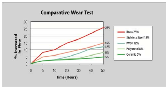
Figure A - Accelerated wear test in Kaolin abrasive. Source: SGS UK
